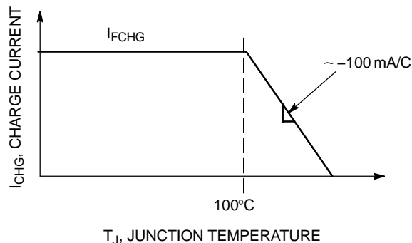
Figure 16. Full Charge Current vs. Junction Temperature
